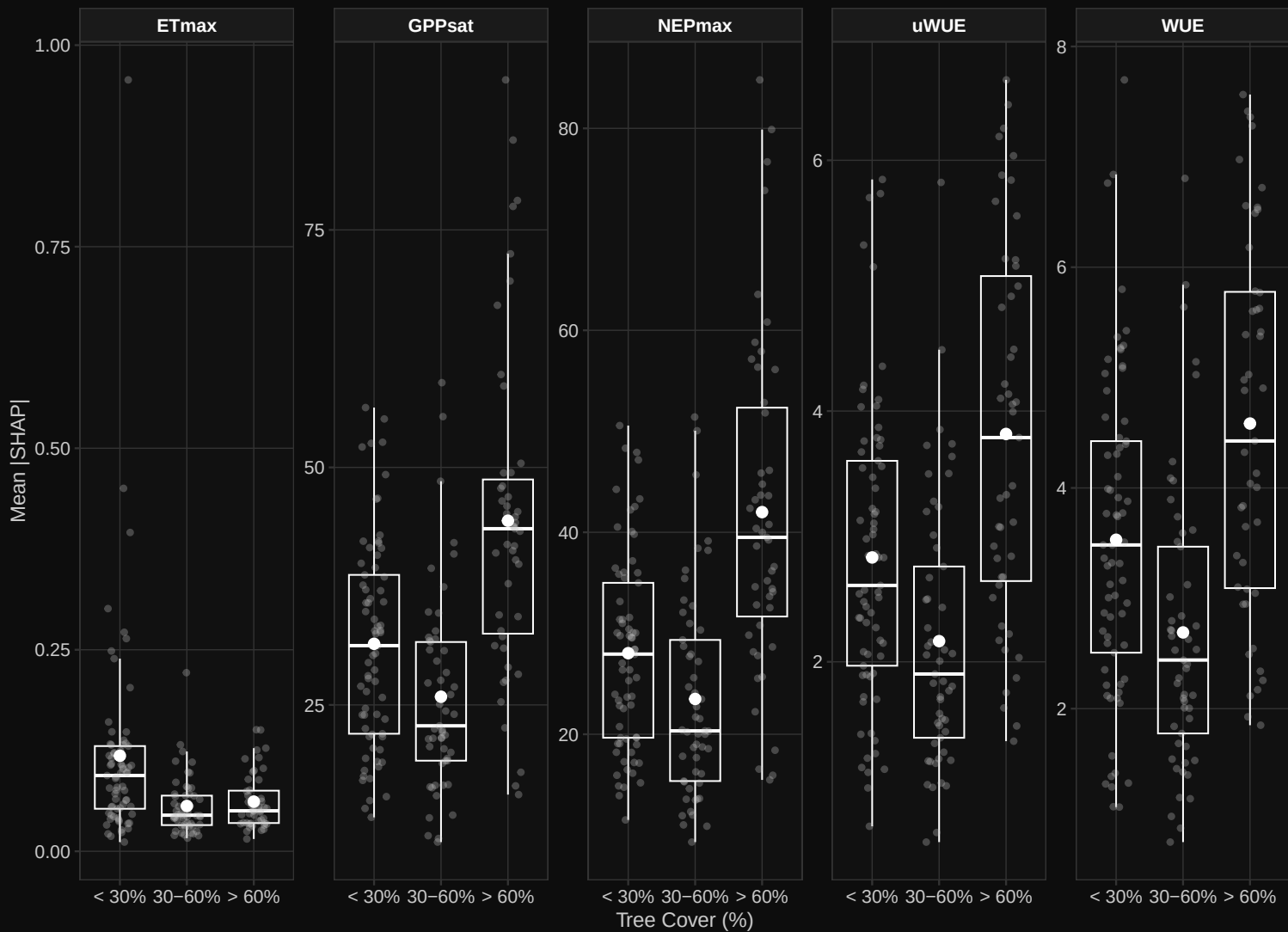
Disturbance SHAP vs Tree Cover – 24m
