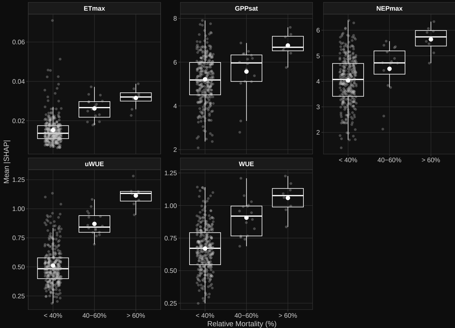
Disturbance SHAP vs Relative Mortality
