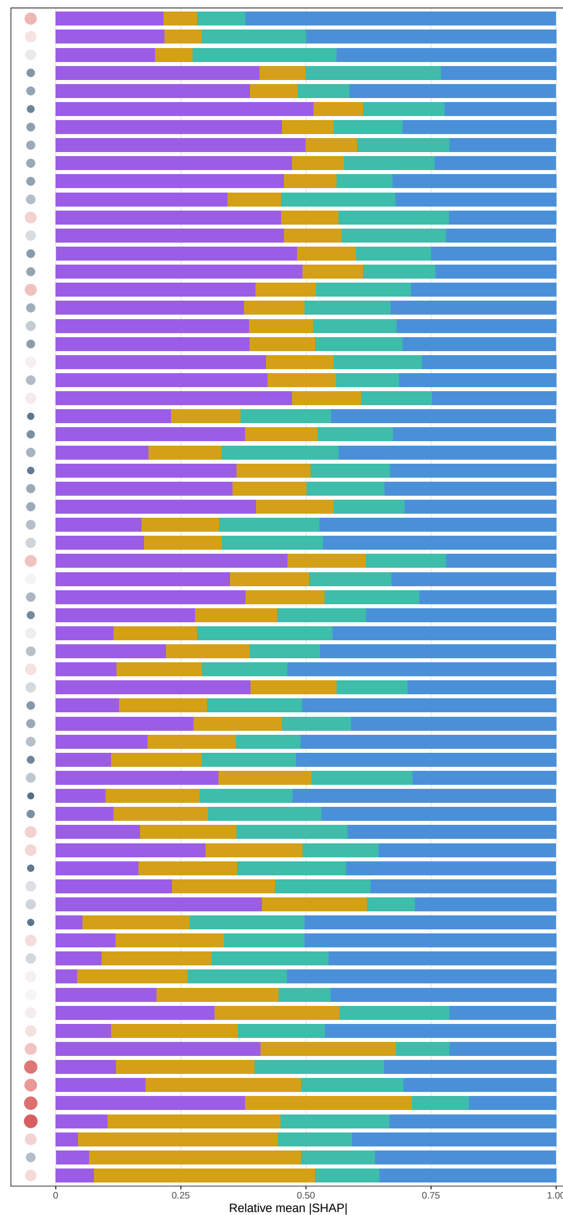
M8 raw (C+T+D+Mem) | 12m window | NEPmax ( \mu\text{mol m}^{-2} \text{s}^{-1} )
