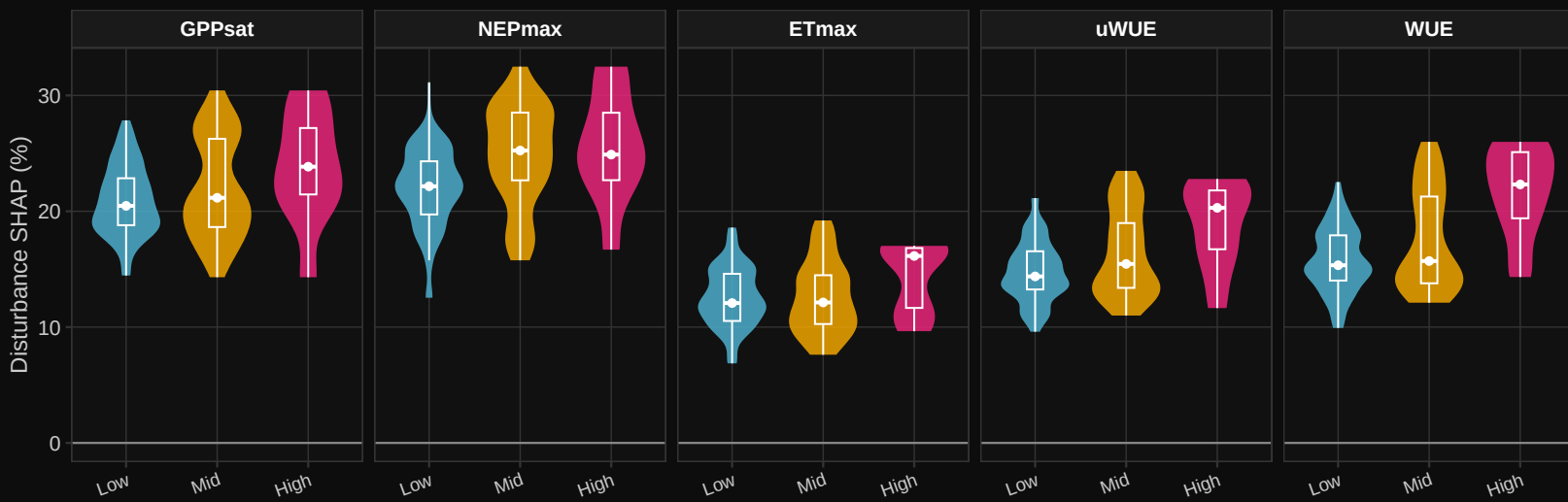
Disturbance SHAP % by Relative Disturbance (M6_anom 24m)
