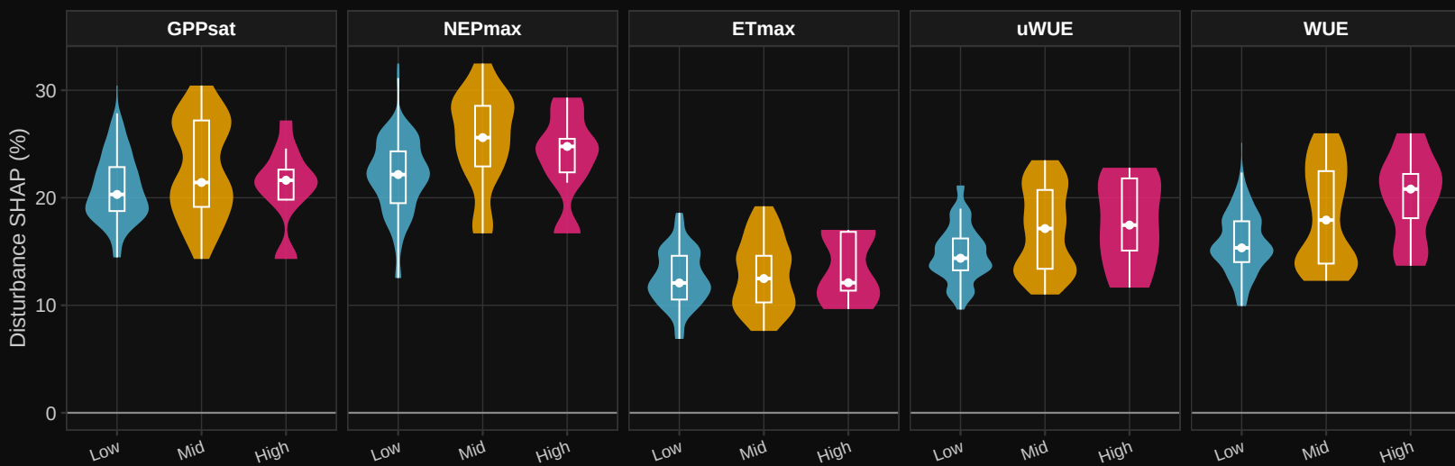
Disturbance SHAP % by Relative Mortality (M6_anom 24m)
