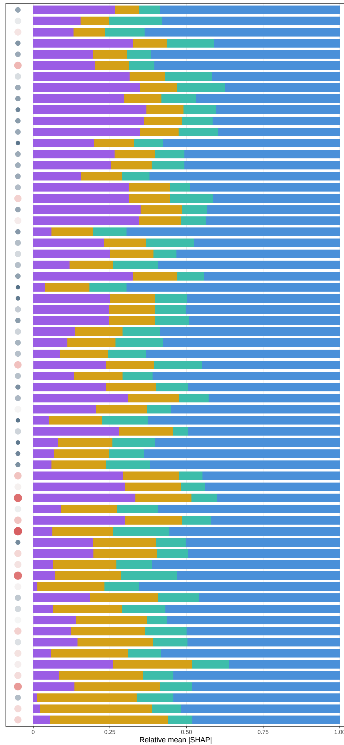
M8 raw (C+T+D+Mem) | 24m window | NEPmax ( \mu\text{mol m}^{-2} \text{s}^{-1} )
