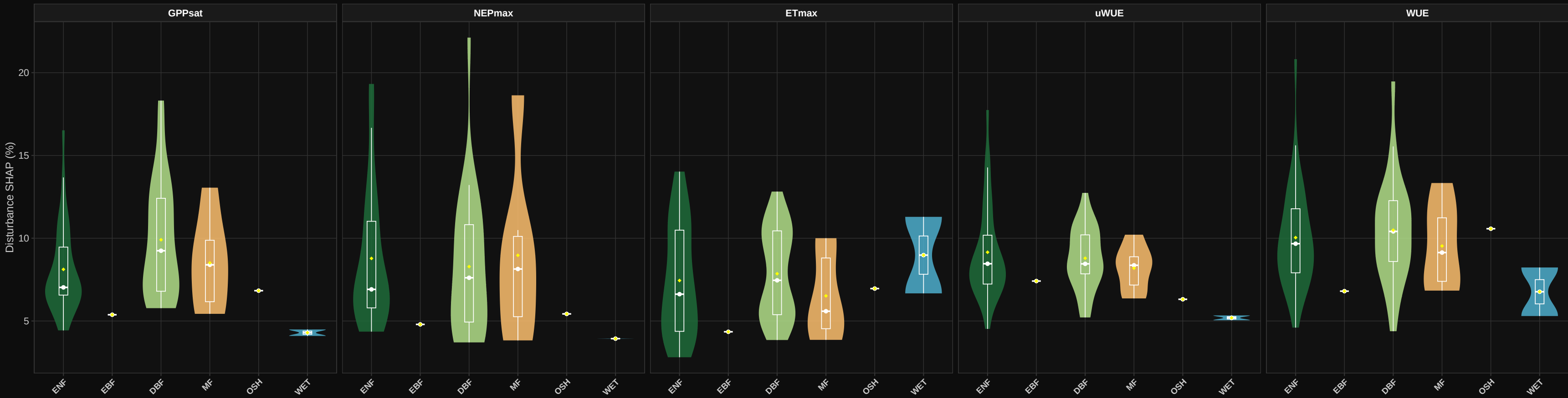
Disturbance SHAP % by IGBP class ... M8 raw (C+T+D+Mem) | 12m
