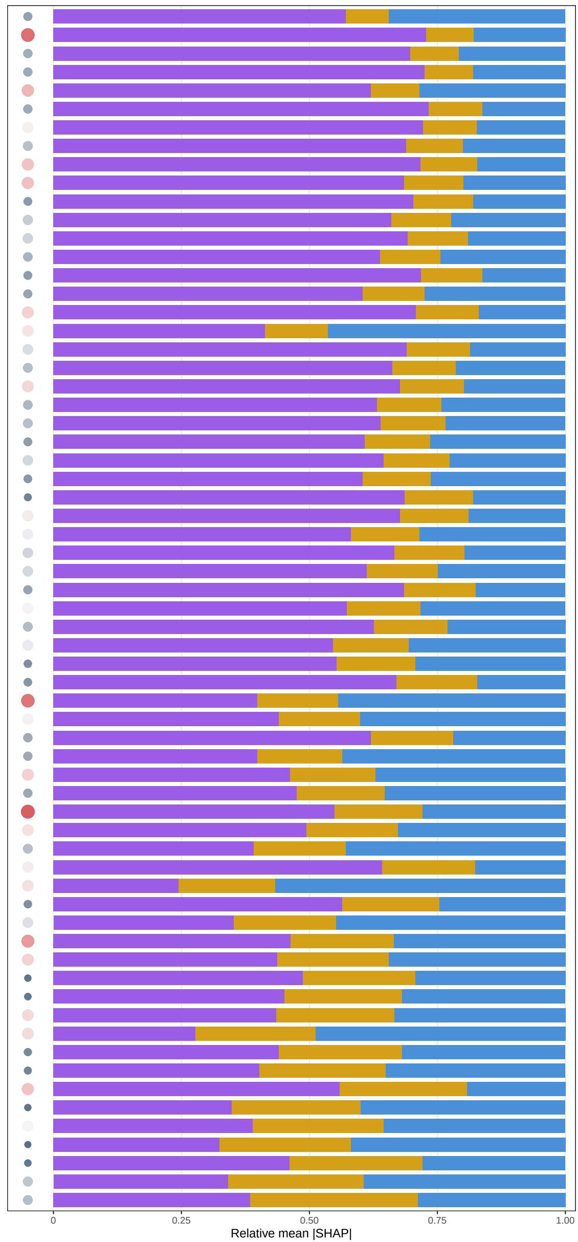
M6 raw (C+T+D+Mem) | 12m window | GPPsat ( \mu\text{mol m}^{-2} \text{s}^{-1} )
