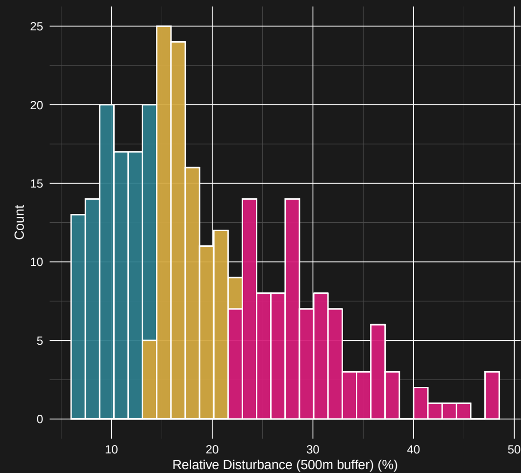
METHOD 1: Tertiles
