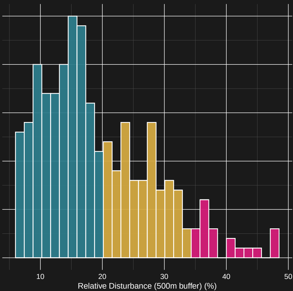
METHOD 2: Equal-Width
