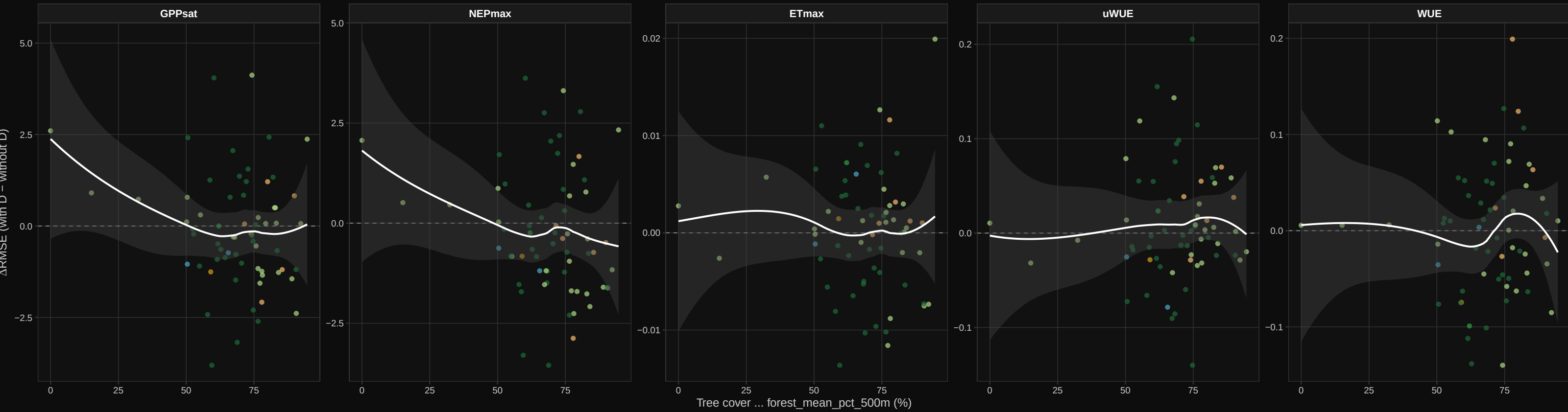
D · Tree cover vs. disturbance SHAP importance
