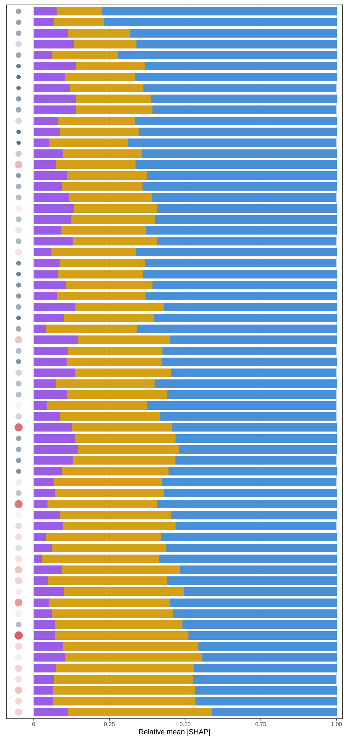
M6 raw (C+T+D+Mem) | 24m window | GPPsat ( \mu\text{mol m}^{-2} \text{s}^{-1} )
