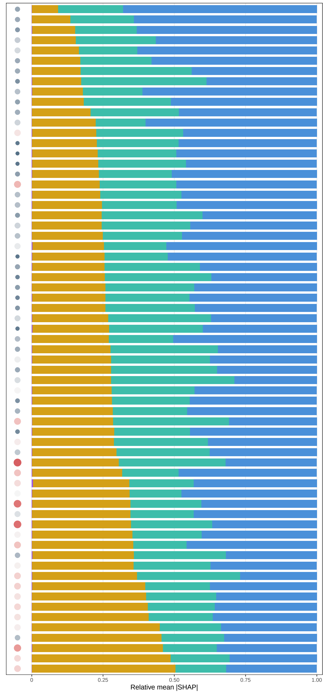
M8 anom (C+T+D+Mem) | 12m window | NEPmax ( \mu\text{mol m}^{-2} \text{s}^{-1} )
