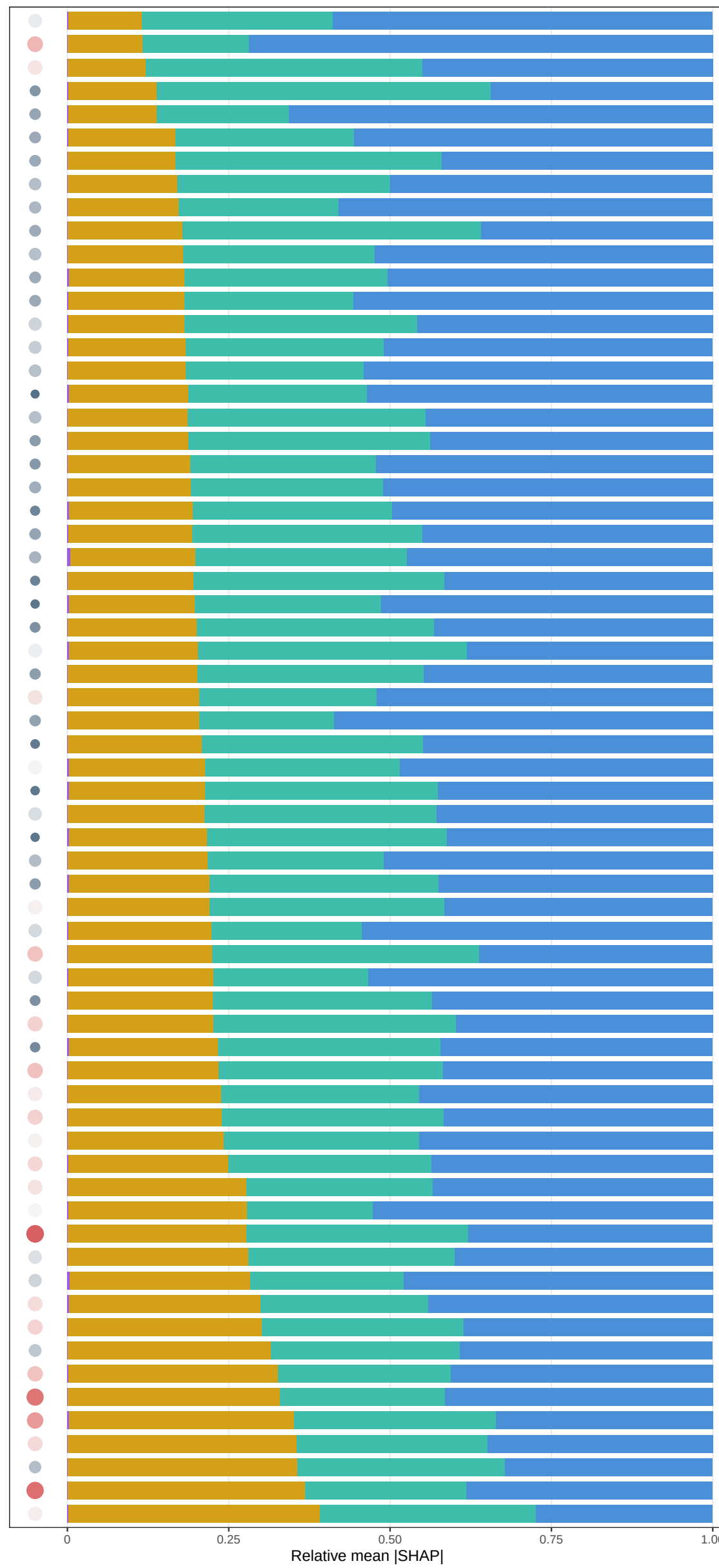
M8 anom (C+T+D+Mem) | 24m window | NEPmax ( \mu\text{mol m}^{-2} \text{s}^{-1} )
