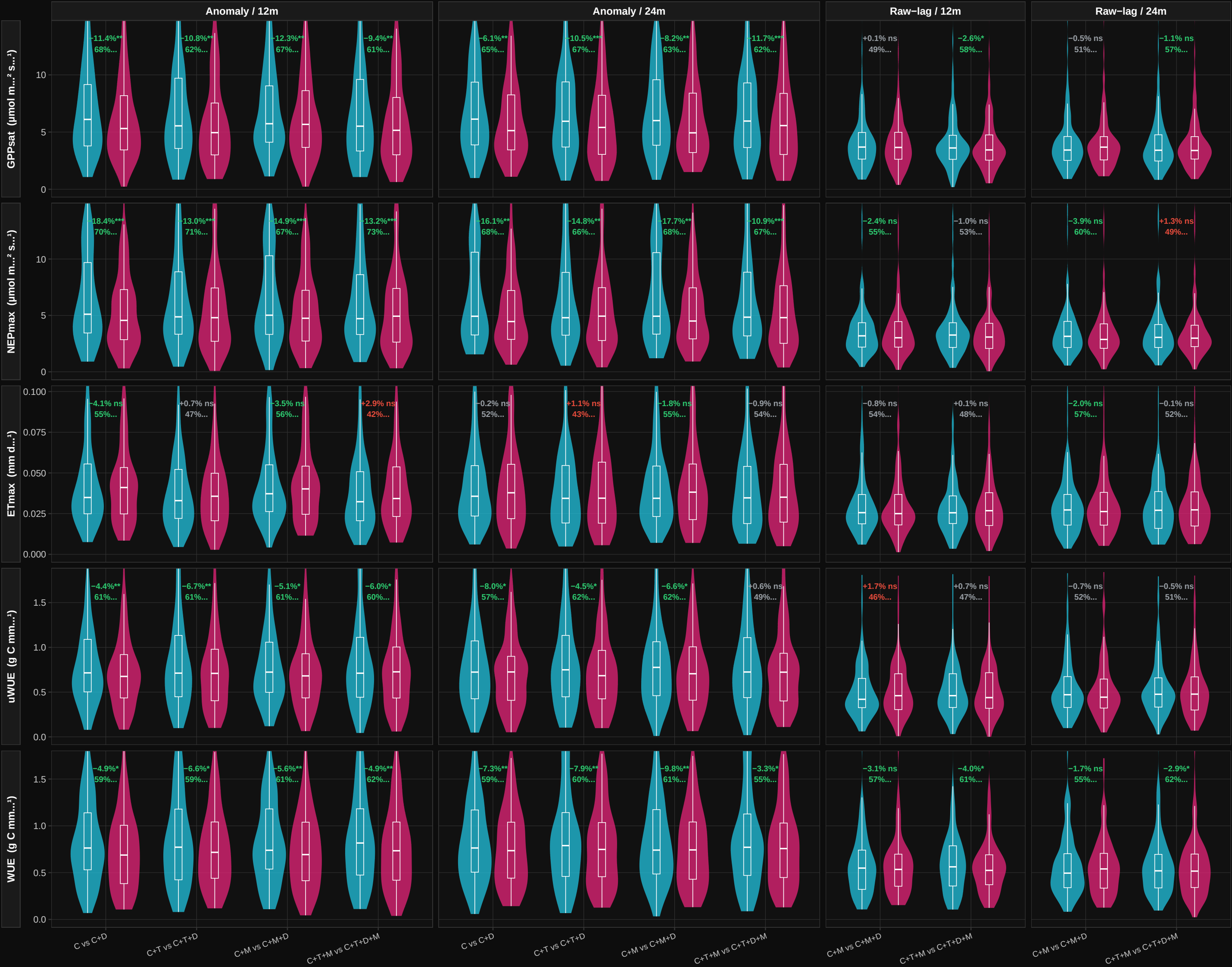
Effect of adding deadwood disturbance on per-site RMSE Paired violin: cyan = without D, pink = with D | LOSO CV | 93 sites | % = MEDIAN PAIRED change in per-site RMSE (negative = less error, green) stars = one-sided paired Wilcoxon, H1: adding D reduces RMSE, BH-FDR within figure (** q<0.001, ** q<0.01, * q<0.05, ns) y axis zoomed to the 95th percentile – no data removed; M1–M4 have no memory term and appear once, under Anomaly
