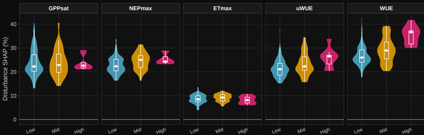
Disturbance SHAP % by Absolute Mortality (M8_anom 24m)
