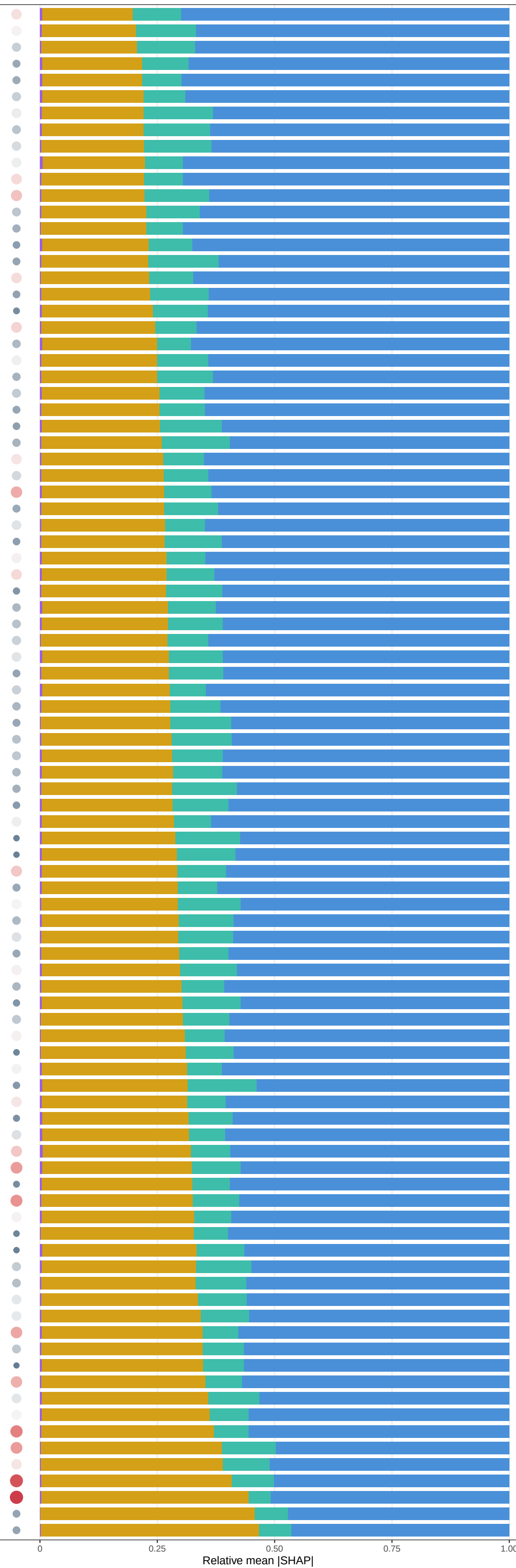
M8 anom (C+T+D+Mem) | 24m window | uWUE (g C mm... 1 )
