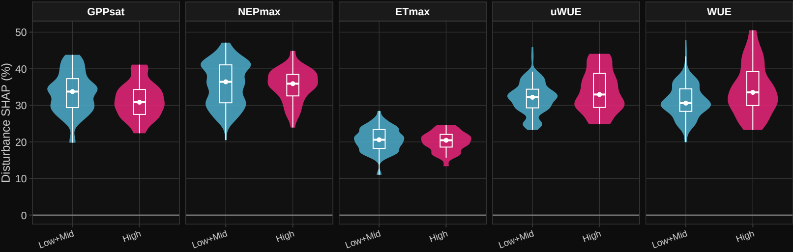
Disturbance SHAP % by Absolute Mortality (M6_anom 12m)
