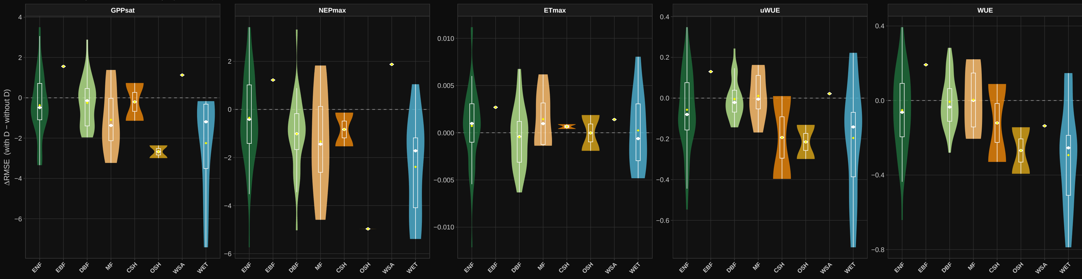
Effect of adding disturbance on per-site RMSE by IGBP class ... M7vsM8_anom_24m
