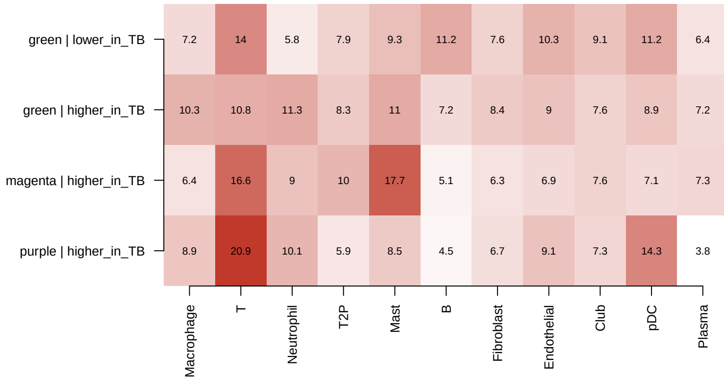
Mean cell-type share of detected module genes (%)
