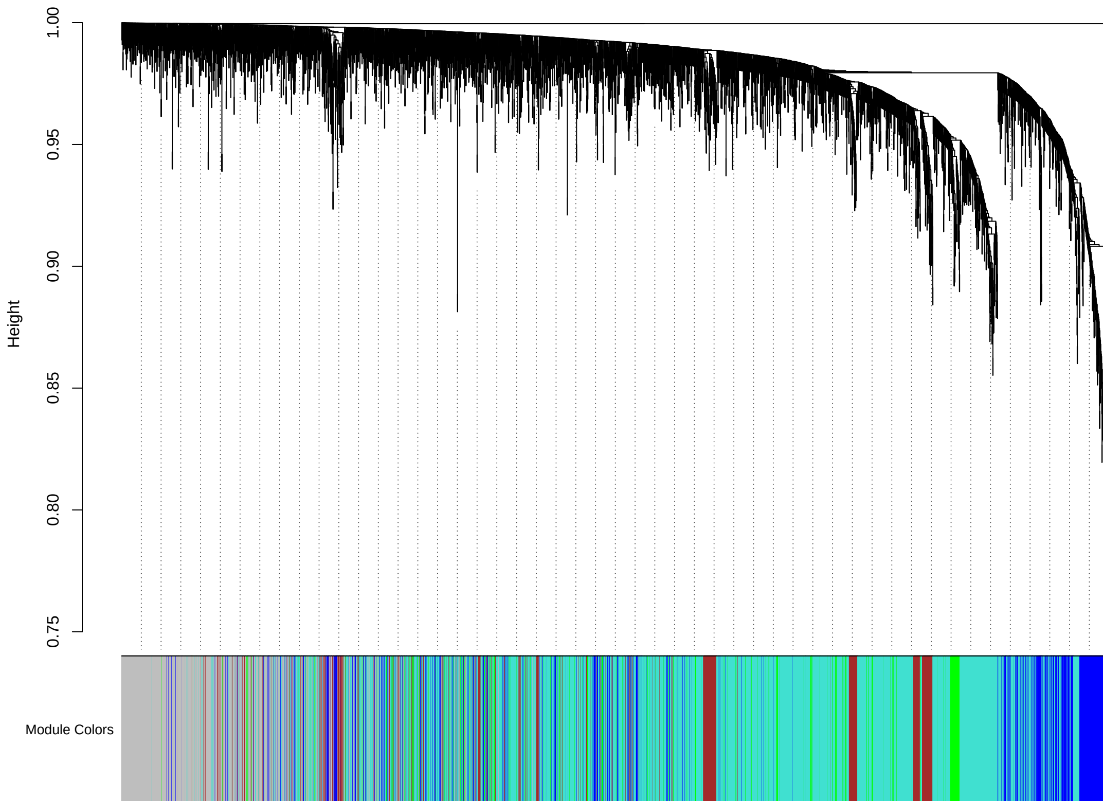
Gene Dendrogram and Module Colors (GSE161829)
