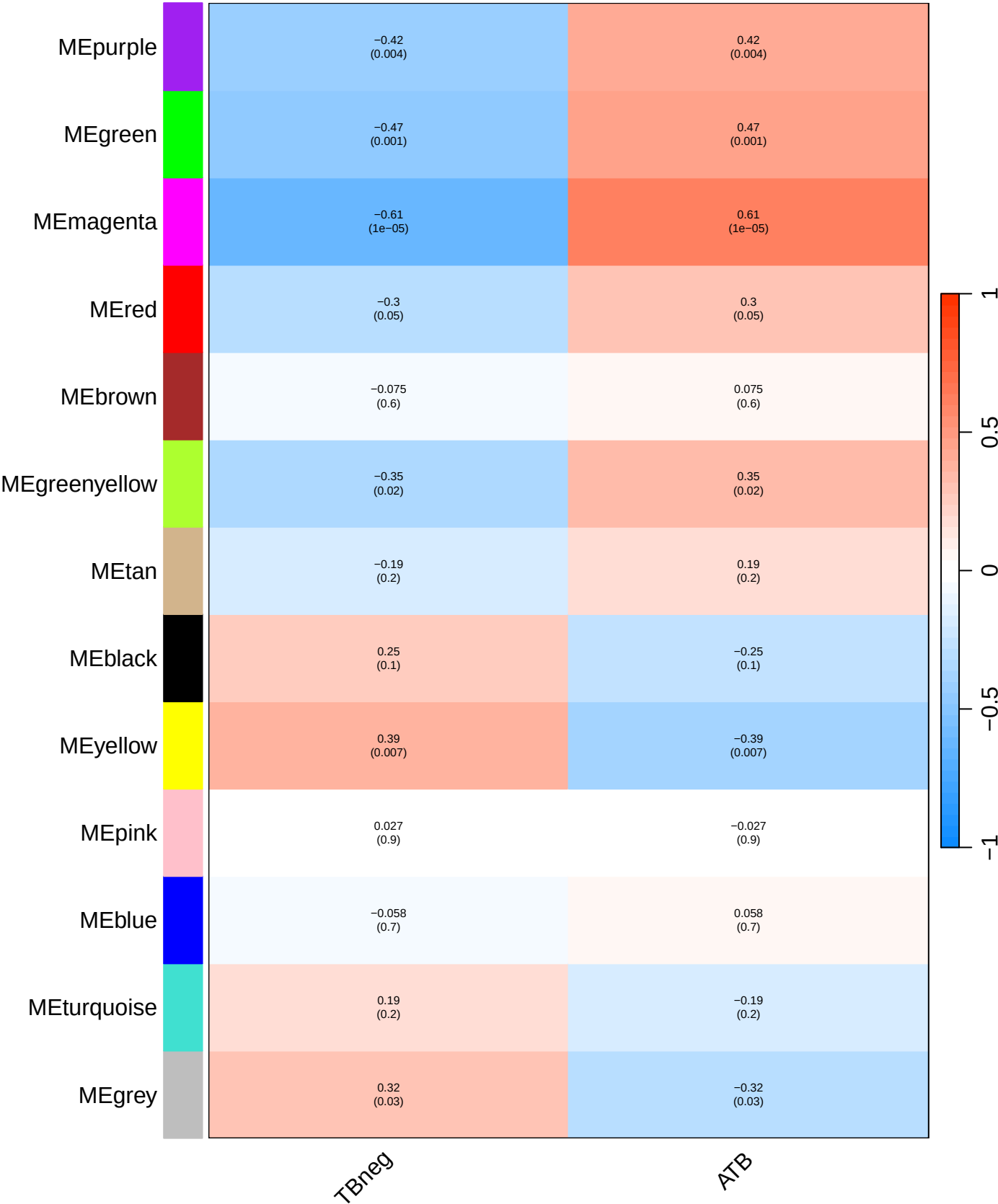
Module–Trait Relationships (GSE161829)
