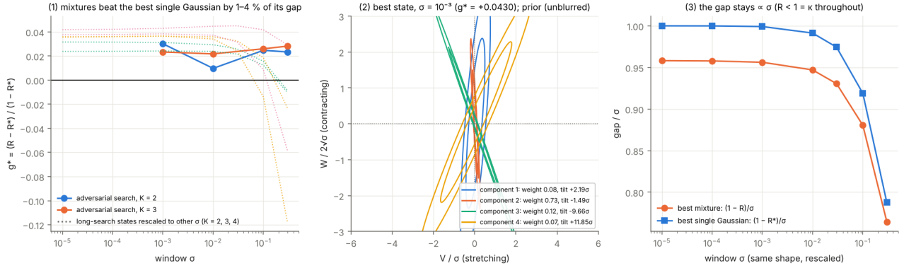
FIG. 3. Mixtures that beat the best Gaussian state (pendulum). (1) Advantage g^* of adversarially optimized mixtures with K = 2 and 3 components, and of long searches rescaled to other \sigma . (2) The best state at \sigma = 10^{-3} ( K = 4 ): four thin components crossing at q = \pi , shown in units of \sigma across and 2\sqrt{\sigma} along. (3) The gap stays proportional to \sigma for the best mixture and for the best Gaussian state.
