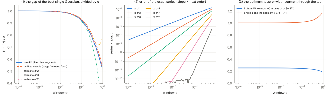
FIG. 2. Best Gaussian state of the pendulum. (1) Gap (1 - R^*)/\sigma of the optimal tilted segment, of the untilted needle, and of truncations of the series (14). (2) Error of the truncated series; the slope equals the next order. (3) Shape of the optimum: tilt from w towards -v in units of \sigma ( \rightarrow 1/4 ) and length in units of 2\sqrt{\sigma} ( \rightarrow 1 ).
