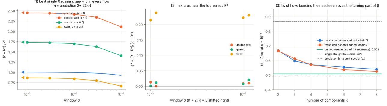
FIG. 5. Resolution gap in four flows. (1) Best Gaussian state: (\kappa - R^*)/\sigma against \sigma ; triangles mark the prediction 2\sqrt{2\beta\kappa} of Proposition 7. (2) Advantage g^* of mixtures near the maximal strain. (3) Twist flow: gap of mixtures with K components, of a bent needle, of the best straight Gaussian state ( \sqrt{3}/2 ) and the prediction 1/2 for a needle that follows the rotation.
