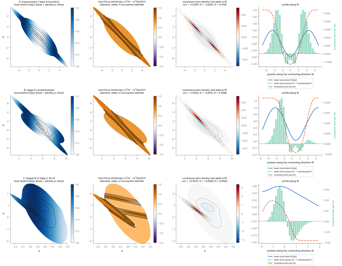
FIG. 1. Mechanism of the covariance term for three pendulum states (rows). Left: local strain \bar{a}(y) and coarse-grained density (contours). Second: local anisotropy of the focus (v^\top H v - w^\top H w) / \text{tr } H ; hatched regions are valleys, where H has a negative eigenvalue. Third: density of the covariance term C (red adds to R ). Right: profile along the contracting direction. The covariance term is positive where the focus is sharp and the strain is strong.
