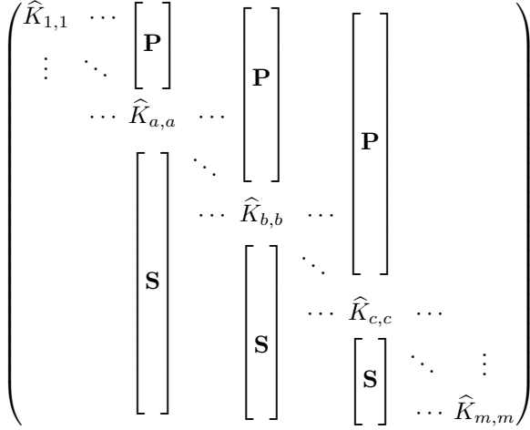
Fig. 2: Coupling of the vectors \hat{\mathbf{y}}_{i_1, i_2, i_3} with the \hat{\mathbf{K}} matrix for a given (a, b, c) .
