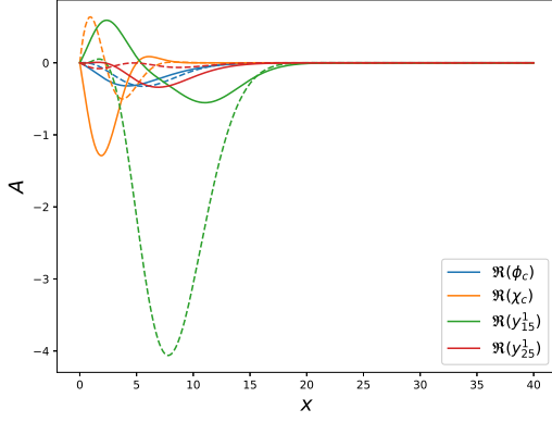
Fig. 4: Numerically evaluated eigenvector fields \phi_c and \chi_c , along with the second-order approximations of stable components \mathbf{y}_{1,5} and \mathbf{y}_{2,5} . The real parts of the fields depicted by solid lines while the imaginary parts are depicted with dashed lines of the same color.
