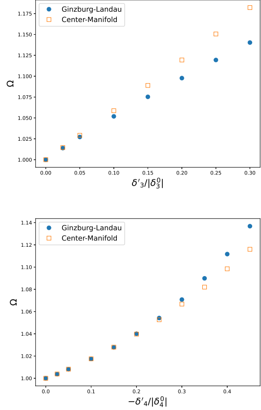
Fig. 5: Comparison of the angular frequencies obtained from the Ginzburg-Landau system, equation (76), and its center-manifold reduction, equation (83) for different values of parameter perturbations. (Top) \delta'_4 = 0 with varying \delta'_3 and, (bottom) \delta'_3 = 0 with varying \delta'_4 . Note the negative sign in the x -axis label in the bottom figure.
