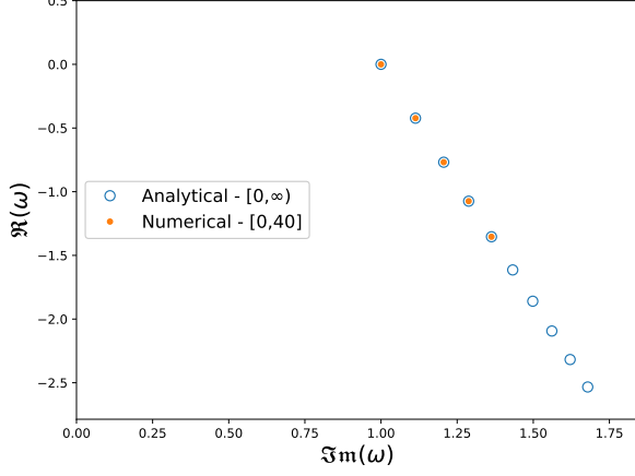
FIG. 1: Comparison of the numerically evaluated spectrum of the Ginzburg-Landau model ( \mathcal{L}_0 ) in the truncated domain with the analytical spectrum in the semi-infinite domain.
