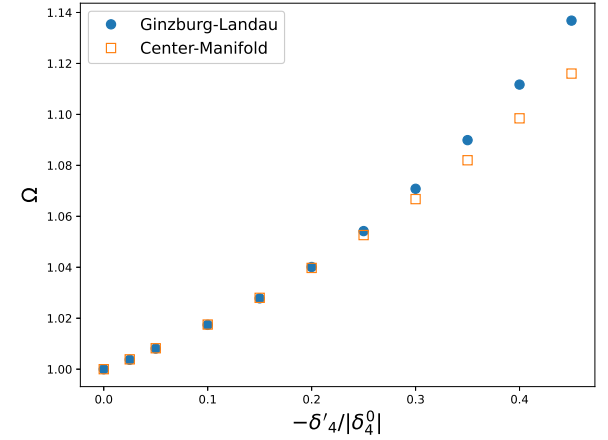
FIG. 3: Comparison of the angular frequencies obtained from the Ginzburg-Landau system, equation (45), and its center-manifold reduction, equation (51) for different values of parameter perturbations. (Top) \delta'_4 = 0 with varying \delta'_3 and, (bottom) \delta'_3 = 0 with varying \delta'_4 . Note the negative sign in the x -axis label in the bottom figure.
