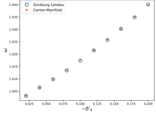
Fig. 6: Variation of the final limit-cycle-oscillation angular frequency due to perturbations of \delta_4 parameter. The empty circles indicate results of the nonlinear simulations of the Ginzburg-Landau system and the filled circles indicate the results of the center manifold approximation.
