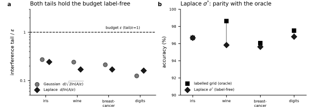
Figure 3: The calibration is not Gaussian-specific. On four public datasets, the Laplace frontier \sigma^* = d/\ln(A/\varepsilon) holds the interference budget label-free and approaches a labelled grid search anchored to the Laplace scale.
