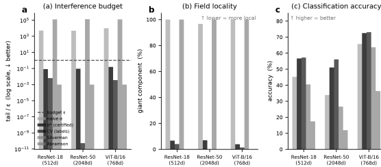
Figure 3. Certified \sigma^* across three frozen backbones (CIFAR-100, \epsilon=0.05 , zero labels). (a) Only \sigma^* holds the interference budget (tail/ \epsilon < 1 ); naive and classical KDE bandwidths overshoot by 10^3 – 10^5 \times . (b) Naive and KDE bandwidths collapse the field into one component; \sigma^* keeps it local. (c) \sigma^* matches the labelled grid-search accuracy label-free, while the KDE selectors trail badly.
