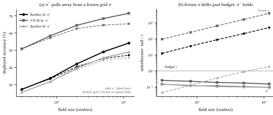
Figure 8. The budget travels--and buys accuracy, on three backbones. A labelled grid-search \sigma is fixed once on the sparse 3-per-class field, then the field densifies to 120 per class. Solid: \sigma^* (label-free, re-measured each stage); dashed: the frozen grid \sigma . (a) \sigma^* pulls away from the frozen bandwidth as the field grows (ResNet-18 +7, ViT-B/16 +6.1, ResNet-50 +3.2 points at full density), tracking a per-stage re-tuned oracle. (b) The frozen bandwidth's interference drifts past the budget (ResNet-18 502 \times , ViT 3865 \times ; ResNet-50 a milder crossing at \approx 2\times ) while \sigma^* holds tail \approx 0.1\epsilon throughout.
