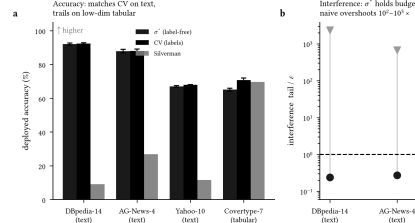
Figure 4. Across four non-image modalities. (a) \sigma^* (label-free) matches the labelled grid search on the three text sets and trails only on low-dimensional tabular data; error bars are \pm 1 s.d. over five seeds. (b) \sigma^* holds the interference budget on every corpus, while the naive bandwidth overshoots by two to three orders of magnitude.
