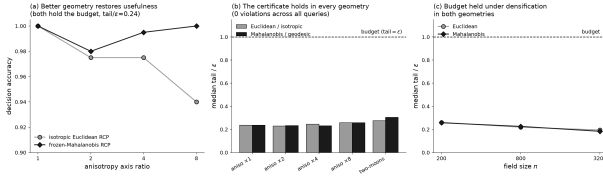
Figure S6: The certificate transfers across frozen geometries. (a) As the anisotropy axis ratio grows, isotropic-Euclidean RCP loses decision accuracy while a frozen-Mahalanobis metric recovers it; both hold the interference budget. (b) Median \text{tail}/\varepsilon stays below the budget in every geometry and configuration, with zero per-query violations. (c) The budget is held under 16\times densification in both the Euclidean and frozen-geometry variants.
