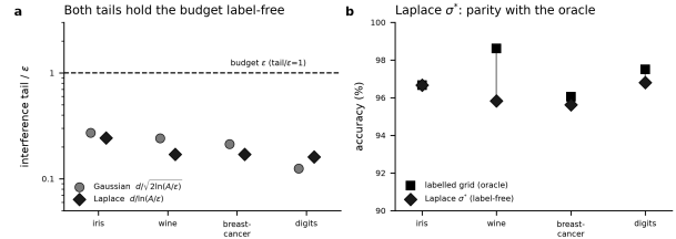
Figure S5: The calibration is not Gaussian-specific. On four public datasets, the Laplace frontier \sigma^* = d/\ln(A/\varepsilon) holds the interference budget label-free and approaches a labelled grid search anchored to the Laplace scale.
