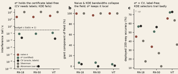
Figure 2. Certified \sigma^* across three frozen backbones (CIFAR-100, \epsilon=0.05 , zero labels). (a) Only \sigma^* holds the interference budget ( \text{tail}/\epsilon < 1 ); naive and classical KDE bandwidths overshoot by 10^3 – 10^5 \times . (b) Naive and KDE bandwidths collapse the field into one component; \sigma^* keeps it local. (c) \sigma^* matches the labelled grid-search accuracy label-free, while the KDE selectors trail badly.
