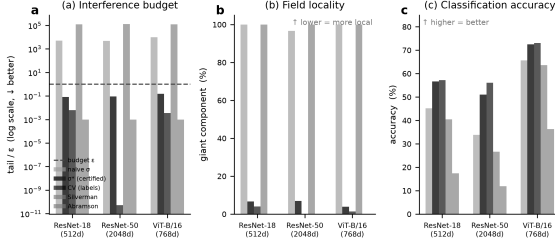
Figure 3. Certified \sigma^* across three frozen backbones (CIFAR-100, \epsilon=0.05 , zero labels). (a) Only \sigma^* holds the interference budget ( \text{tail}/\epsilon < 1 ); naive and classical KDE bandwidths overshoot by 10^3\text{--}10^5\times . (b) Naive and KDE bandwidths collapse the field into one component; \sigma^* keeps it local. (c) \sigma^* matches the labelled grid-search accuracy label-free, while the KDE selectors trail badly.
