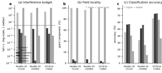
Figure 3. Certified \sigma^* across three frozen backbones (CIFAR-100, \epsilon=0.05 , zero labels). (a) Only \sigma^* holds the interference budget ( \text{tail}/\epsilon < 1 ); naive and classical KDE bandwidths overshoot by 10^2 – 10^5 \times . (b) Naive and KDE bandwidths collapse the field into one component; \sigma^* keeps it local. (c) \sigma^* matches the labelled grid-search accuracy label-free, while the KDE selectors trail badly.
