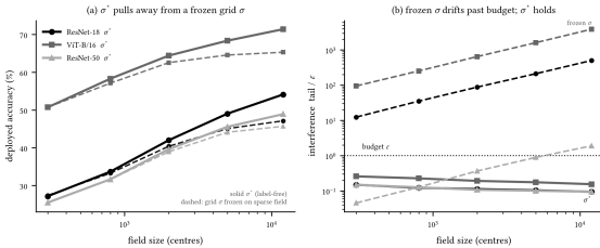
Figure 8. The budget travels--and buys accuracy, on three backbones.
