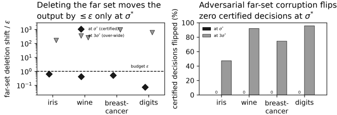
Figure 1: Certified output locality. (a) Deleting all far sources moves the output by at most \epsilon at \sigma^* on all four datasets; 3\sigma^* overshoots by two to three orders of magnitude. (b) Under admissible far-set corruption, certified-stable decisions do not flip at \sigma^* , versus 47–96% at 3\sigma^* .
