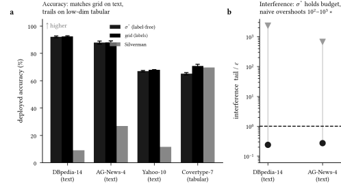
Figure 3: Cross-modal replication. (a) \sigma^* matches labelled grid search on three text datasets and trails on low-dimensional tabular data; error bars are \pm 1 s.d. over five seeds. (b) It holds the budget on every corpus, while the naive bandwidth overshoots by two to three orders of magnitude.
