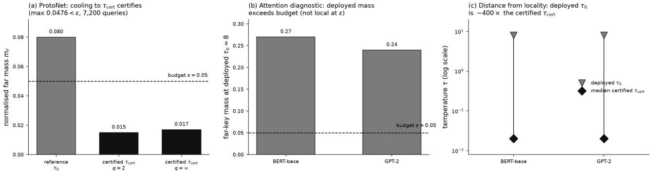
Figure 5: The operational Gibbs certificate. (a) A conv-4 prototypical network: cooling from the reference temperature \tau_0 to the certified \tau_{\text{cert}} pulls the normalised far mass from 0.080 below the budget \epsilon = 0.05 (means 0.015 for q = 2 , 0.017 for q = \infty ; maximum 0.0476 < \epsilon over 7,200 queries). (b) Pretrained attention is the diagnostic boundary: at the deployed \tau_0 = \sqrt{d_k} = 8 the far-key mass is 0.27 (BERT-base) and 0.24 (GPT-2), above budget, so deployed attention is not concentrated on its designated near-key set at \epsilon = 0.05 . (c) The per-query certified temperatures have median \approx 0.02 , roughly 400\times colder than deployment: meeting the budget would require radically sharper attention, a diagnostic scale rather than a deployable retuning.
