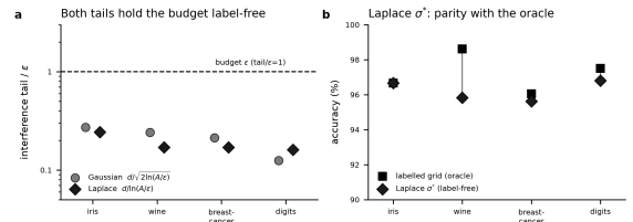
Figure 5. The calibration is not Gaussian-specific. On four public datasets the Laplace frontier \sigma^* = d/\ln(A/\epsilon) behaves like the Gaussian one. (a) Both tails hold the interference budget label-free (tail/ \epsilon < 1 ). (b) The Laplace \sigma^* reaches parity with a labelled grid search anchored to the Laplace scale.
