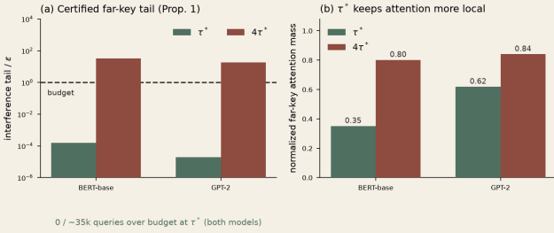
Figure 6. Attention inherits the certificate. On real query/key vectors from BERT-base and GPT-2 (all sampled heads, 360 keys each). (a) At the certified temperature ^* the far-key interference tail is far below budget (mean <10^{-3}\epsilon ; zero of 35,000 queries per model exceed it) and blows up 18–33 \times at 4^* . (b) \tau^* holds attention markedly more local than an over-wide temperature.
