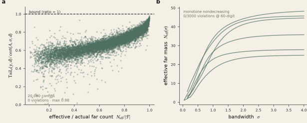
Figure 3. Independent verification of the two load-bearing results. (a) Tail-bound tightness over 20,000 random far configurations: the ratio stays below one everywhere (max 0.98, zero violations), nearing one only as N_{\text{eff}}/|F| \rightarrow 1 . (b) N_{\text{eff}}(\sigma) is monotone nondecreasing (Proposition 2), zero violations at 60-digit precision over 3,000 trials.
