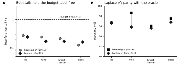
Figure S5: The calibration is not Gaussian-specific. On four public datasets, the Laplace frontier \sigma^* = d/\ln(A/\varepsilon) holds the interference budget label-free and approaches a labelled grid search anchored to the Laplace scale.
