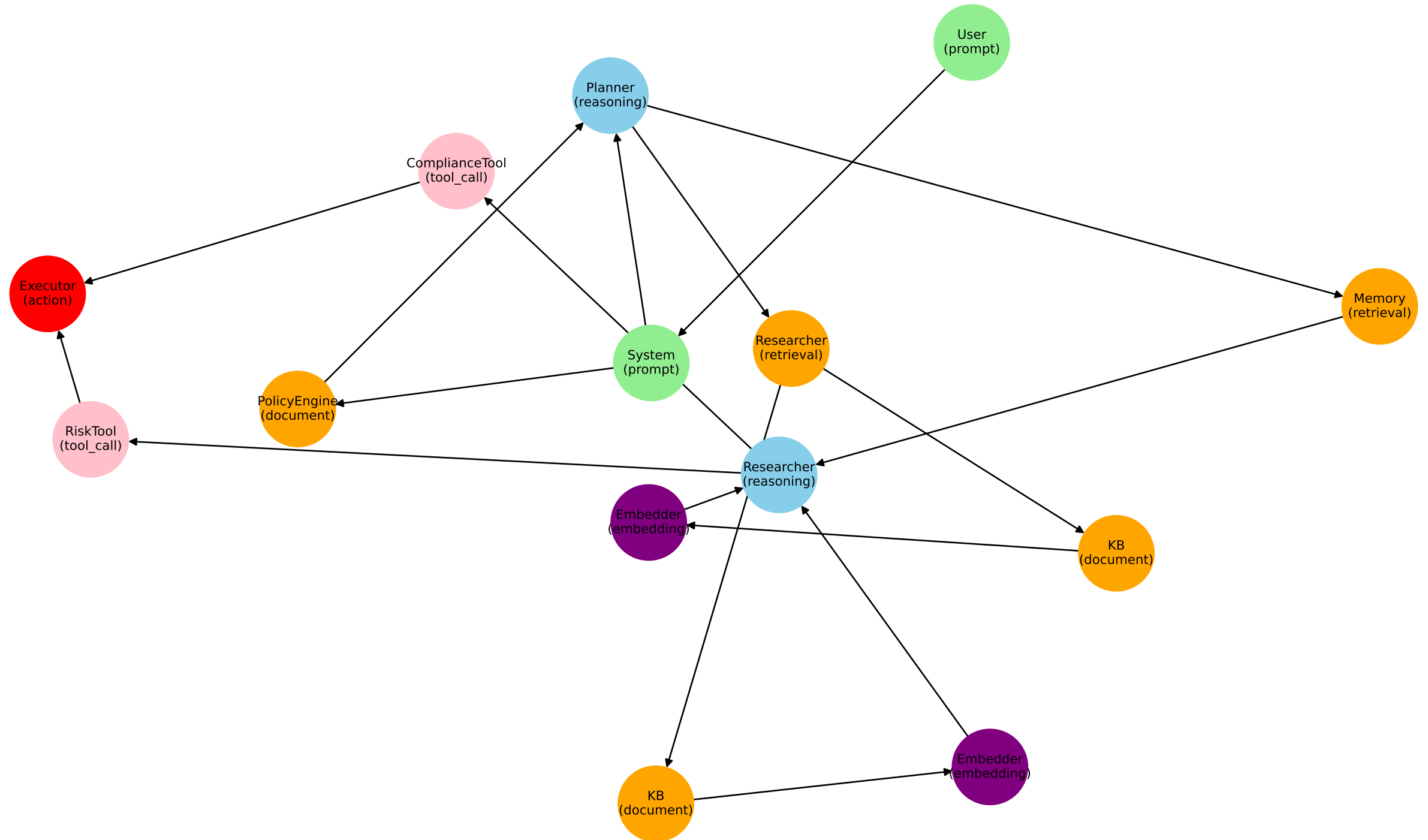
Multi-Layer Provenance Graph (MLPG)
