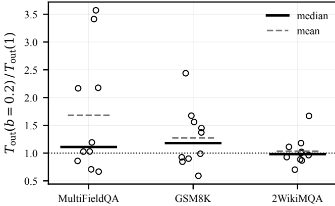
Fig. 2. Per-instance output expansion at b = 0.2 relative to b = 1.0 . Each circle is one instance. The distribution is heavy-tailed on MultiFieldQA: the mean (dashed) is pulled well above the median (solid) by four instances, while three others contract.
