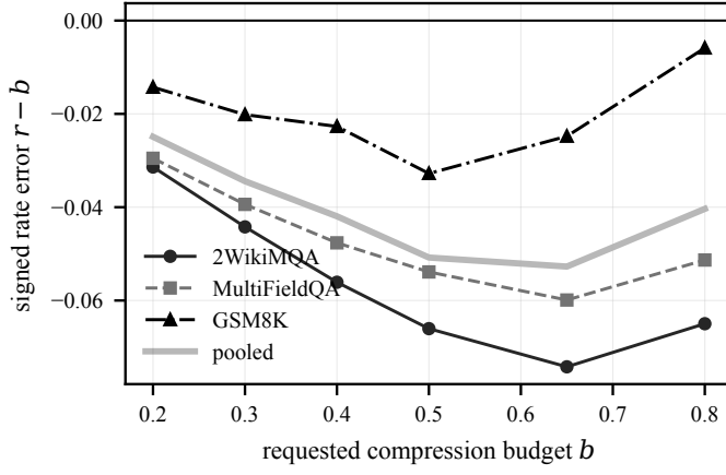
Fig. 1. Signed rate error r - b against requested budget, by family and pooled. The error is negative at every budget, is largest in magnitude near b = 0.65 , and differs by roughly a factor of three between 2WikiMQA and GSM8K.
