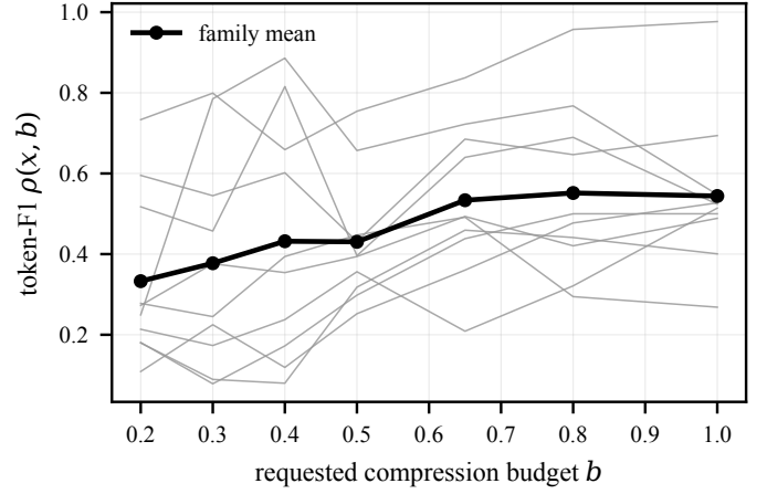
Fig. 3. Per-instance quality against requested budget on MultiFieldQA, the one family with no validity problems. Grey lines are individual instances, black is the family mean. The spread between instances is visible; Section III-C shows it is not separable from sampling noise at k = 3 .
