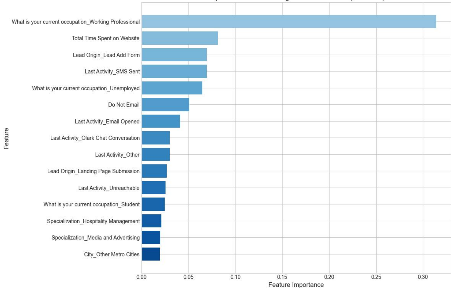
Top Features Influencing Lead Conversion (XGBoost)
