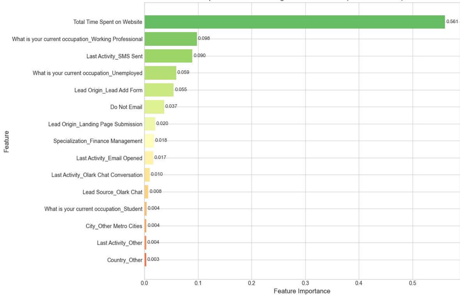
Top Features Influencing Lead Conversion (Random Forest)
