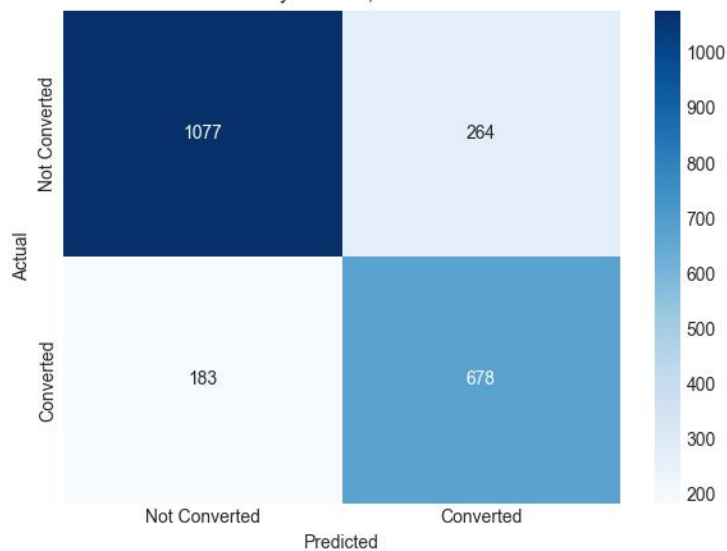
XGBoost Accuracy: 0.7970, F1: 0.7521
