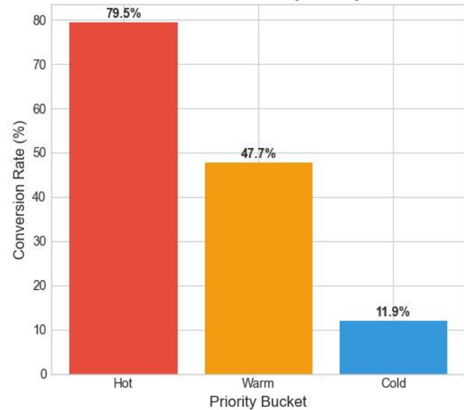
Actual Conversion Rate by Priority Bucket
