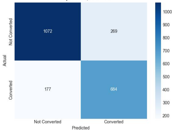
Random Forest Accuracy: 0.7975, F1: 0.7541
