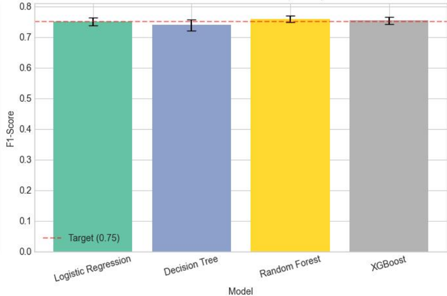
Cross-Validation F1-Score (5-Fold)
