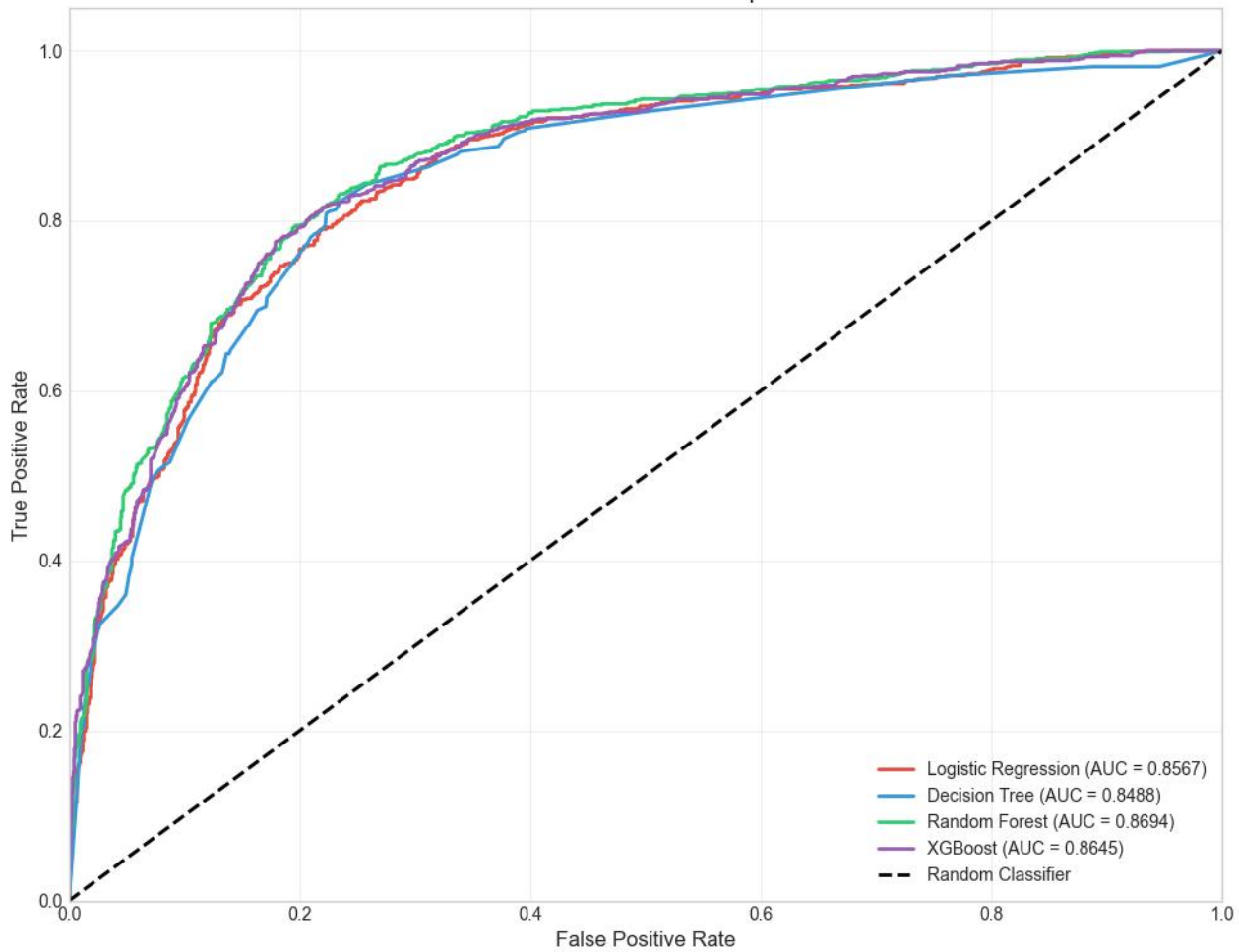
ROC Curves - Model Comparison
