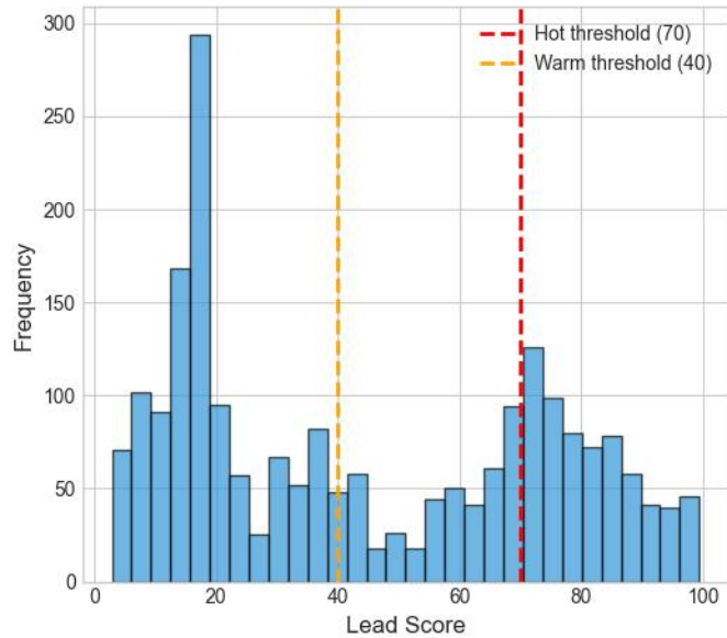
Lead Score Distribution
