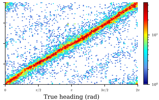
Rotation-Augmented Dataset
