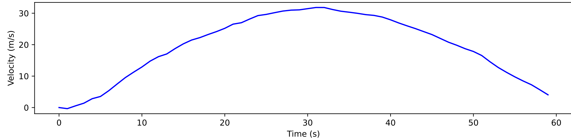
Kalman Filter Output ( \hat{v}_k )
