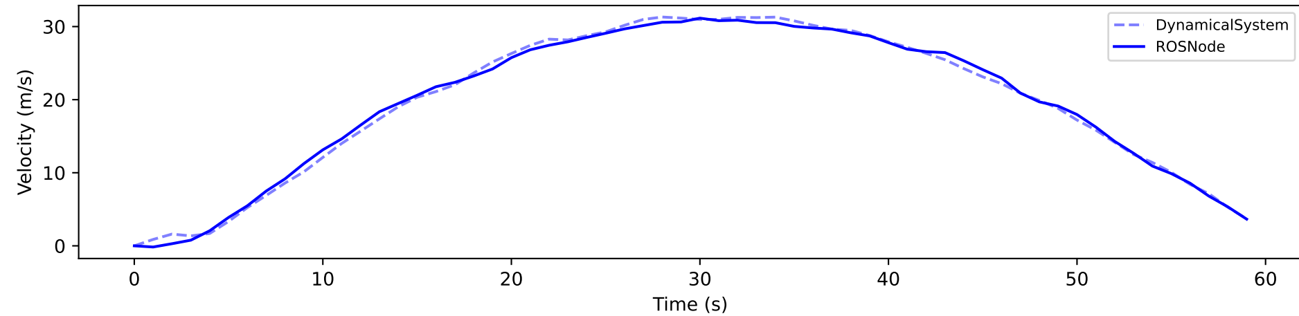
Kalman Filter Output ( \hat{x}_k )
