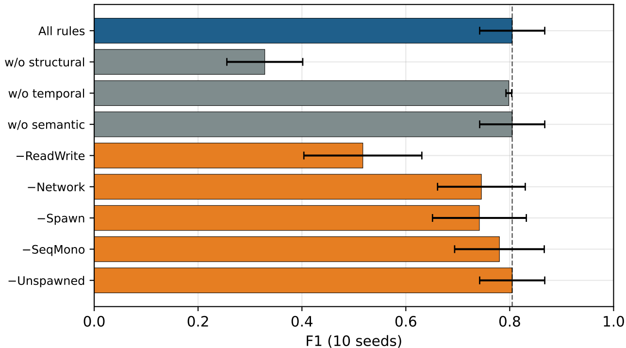
Rule ablation and leave-one-rule-out (dashed line = all-rules baseline)
