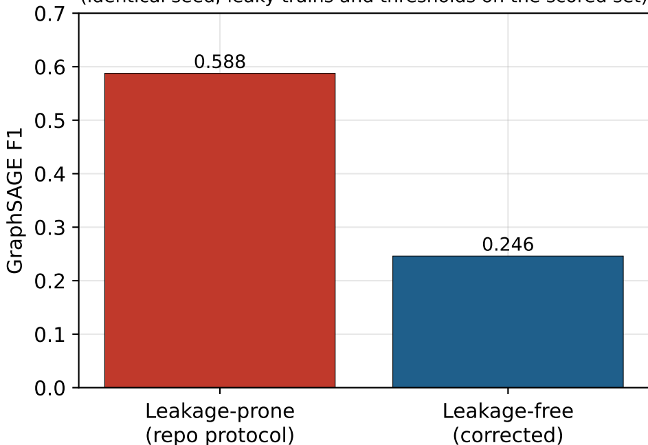
Effect of evaluation leakage on GraphSAGE F1 (identical seed; leaky trains and thresholds on the scored set)
