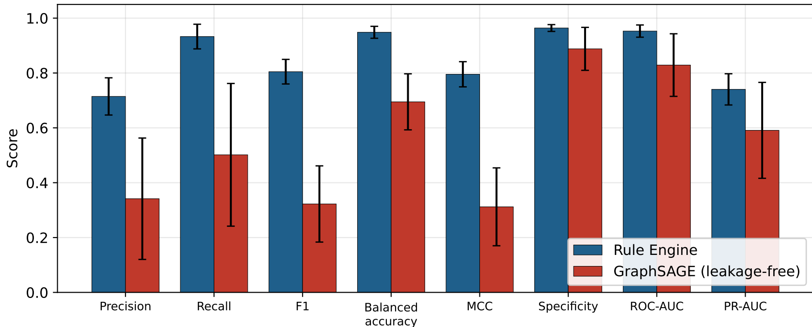
Synthetic controlled poisoning: Rule Engine vs GraphSAGE (10 seeds, mean and 95% CI; corrected final-graph protocol)
