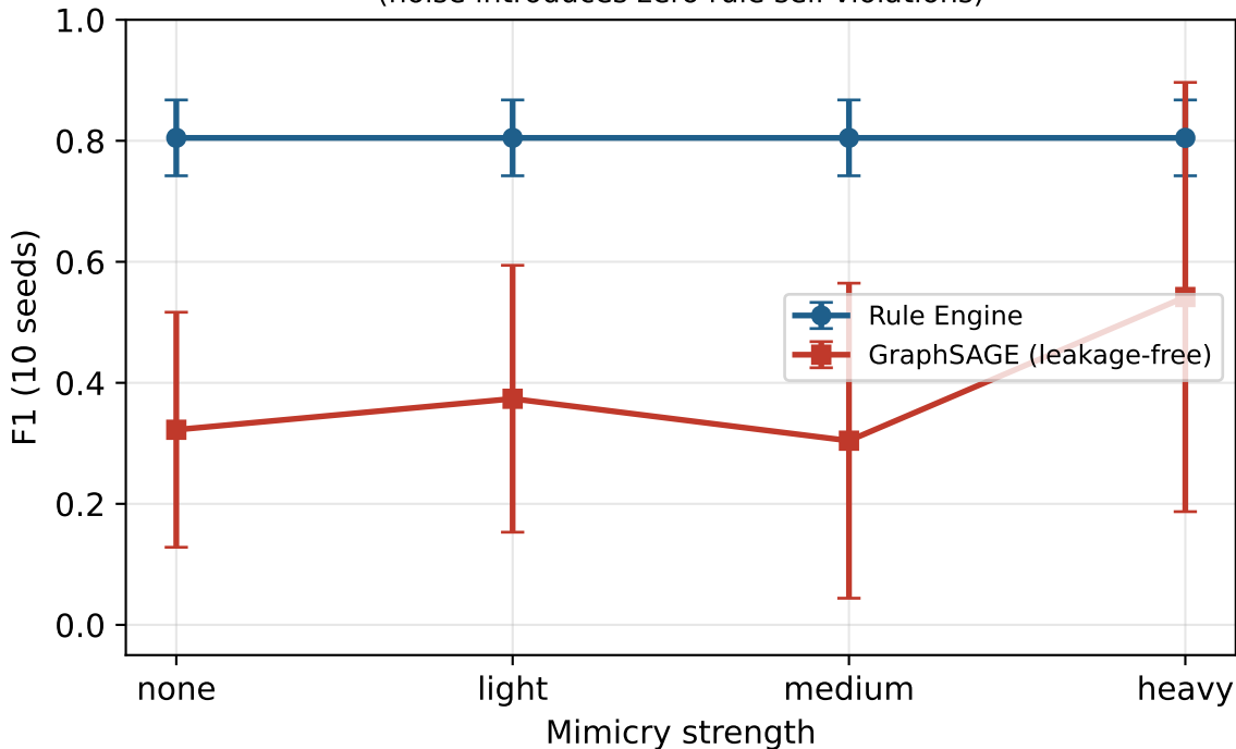
Robustness to invariant-preserving mimicry (noise introduces zero rule self-violations)
