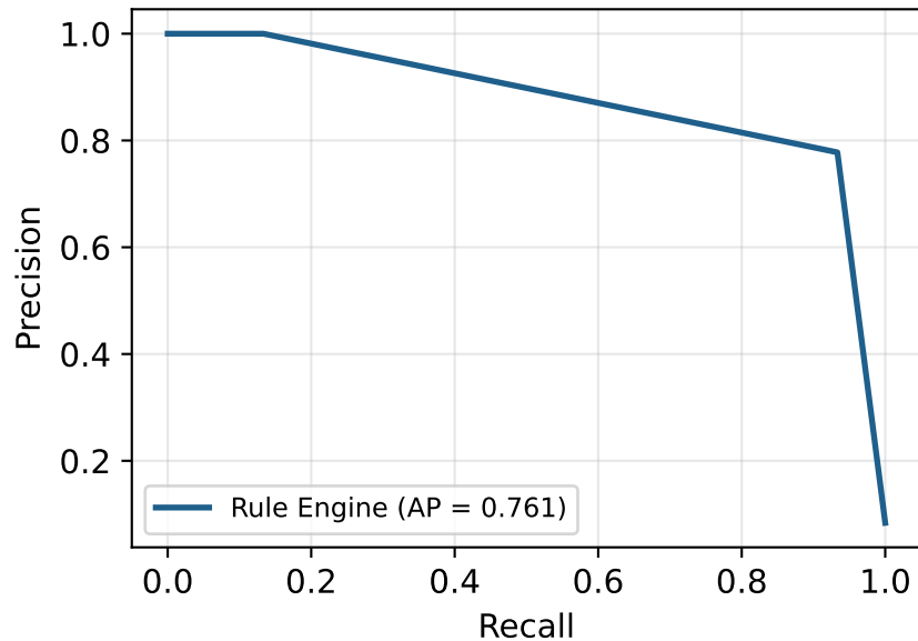
Precision-Recall
