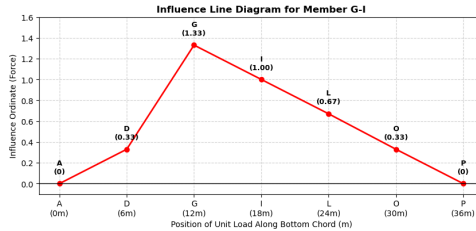
Fig. 1.2.8.2. Correct influence line for axial force in member G - I .
