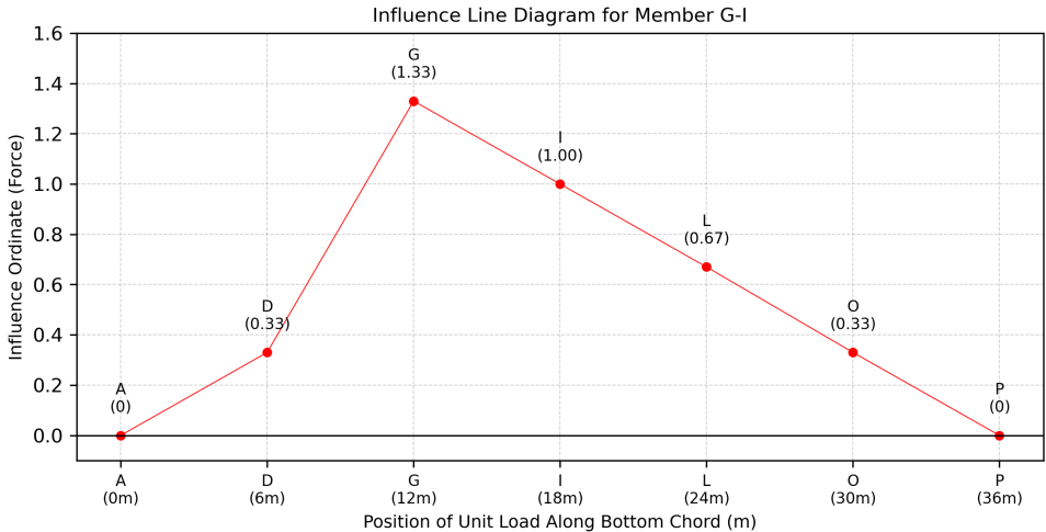
Fig. 4. Influence line graph
