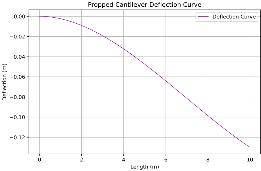
Fig. 5. Propped cantilever and support settlement.
