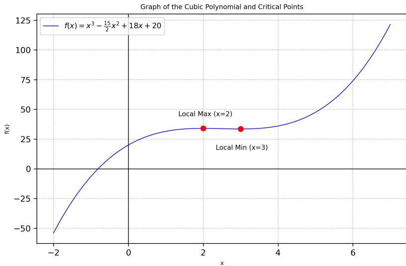
Fig. 6. Graph of the cubic function.
